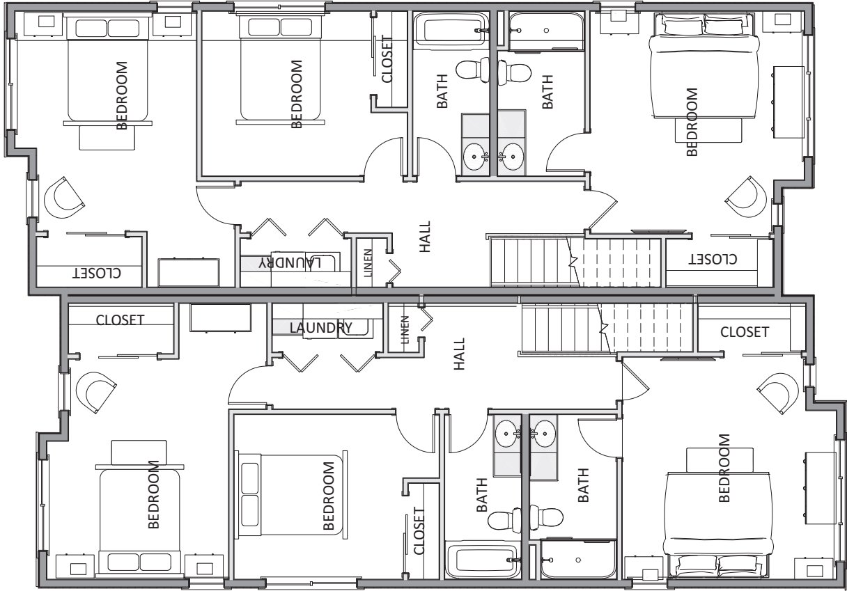
2nd Floor
