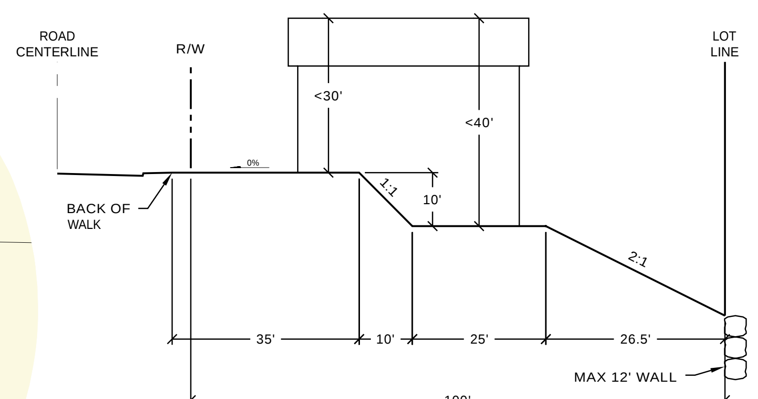
TYPICAL DAYLIGHT LOT CROSS SECTION NOT TO SCALE
