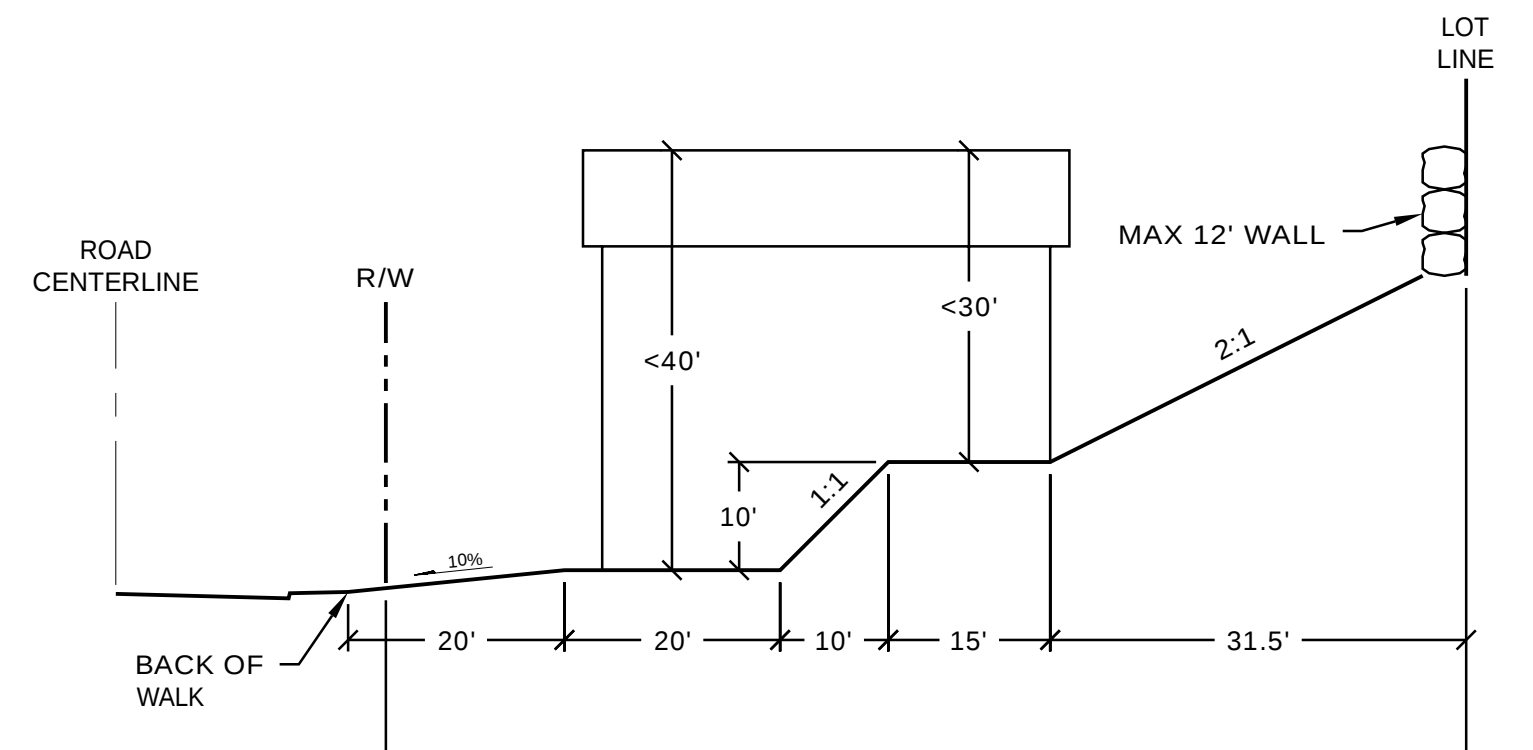
TYPICAL TUCK UNDER CROSS SECTION NOT TO SCALE
