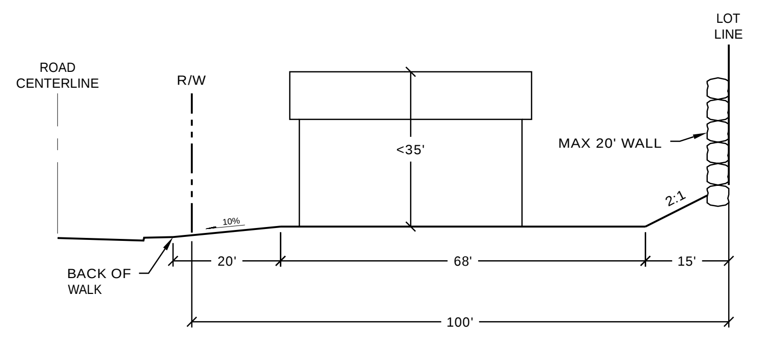
TYPICAL FLAT CROSS SECTION NOT TO SCALE
