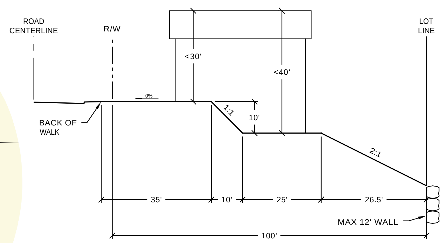
TYPICAL DAYLIGHT LOT CROSS SECTION NOT TO SCALE
