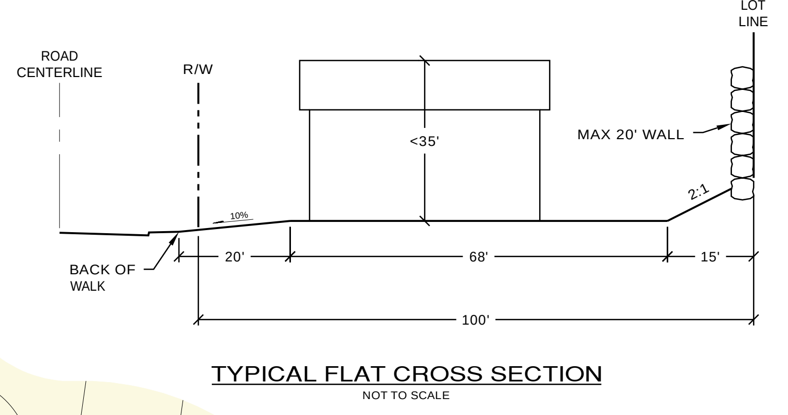
TYPICAL FLAT CROSS SECTION NOT TO SCALE
