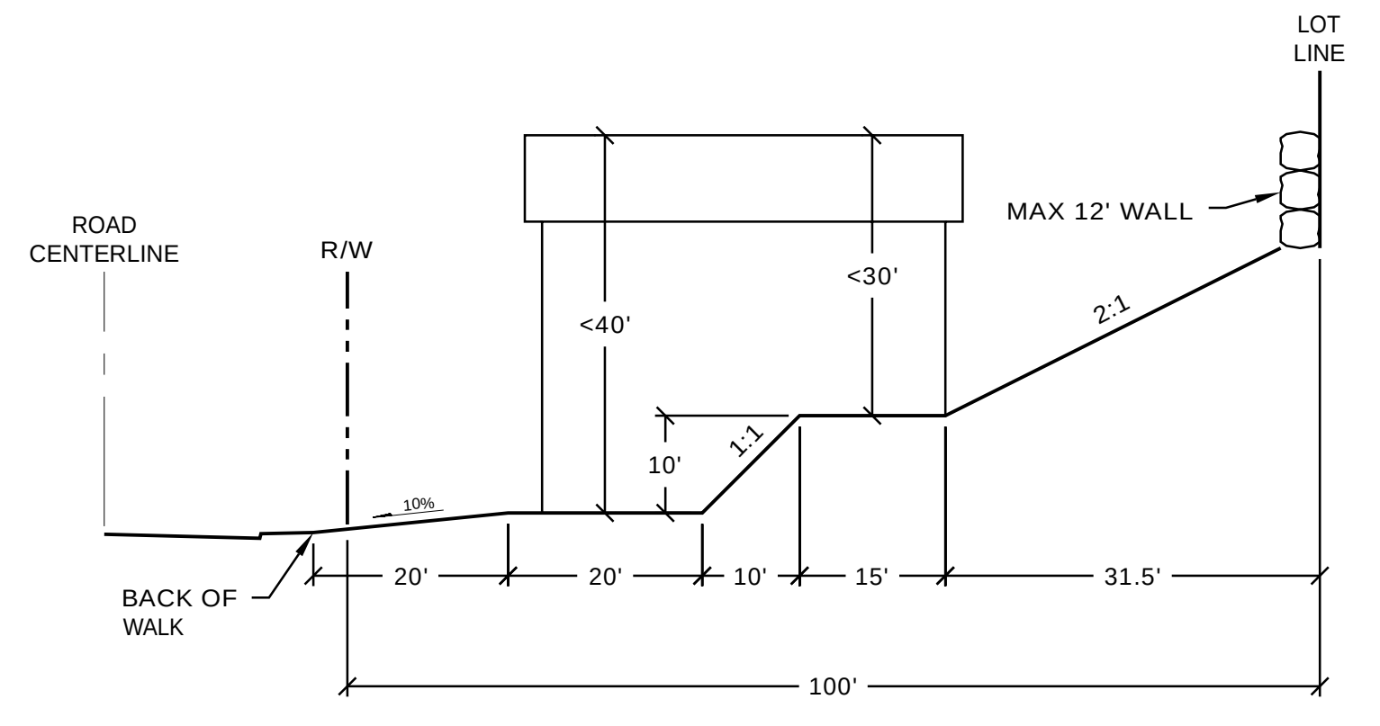
TYPICAL TUCK UNDER CROSS SECTION NOT TO SCALE
