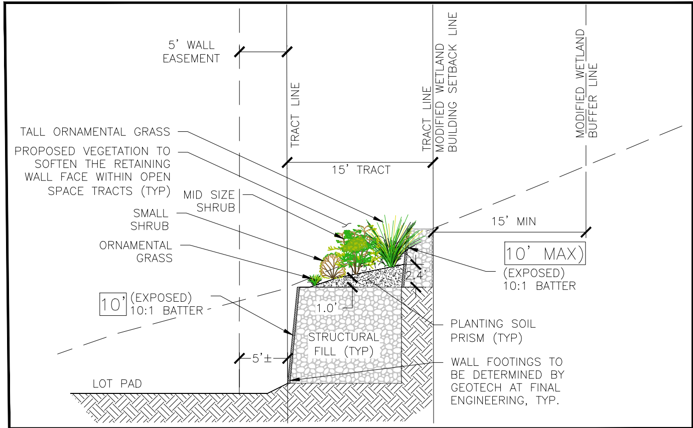
SECTION F-F
