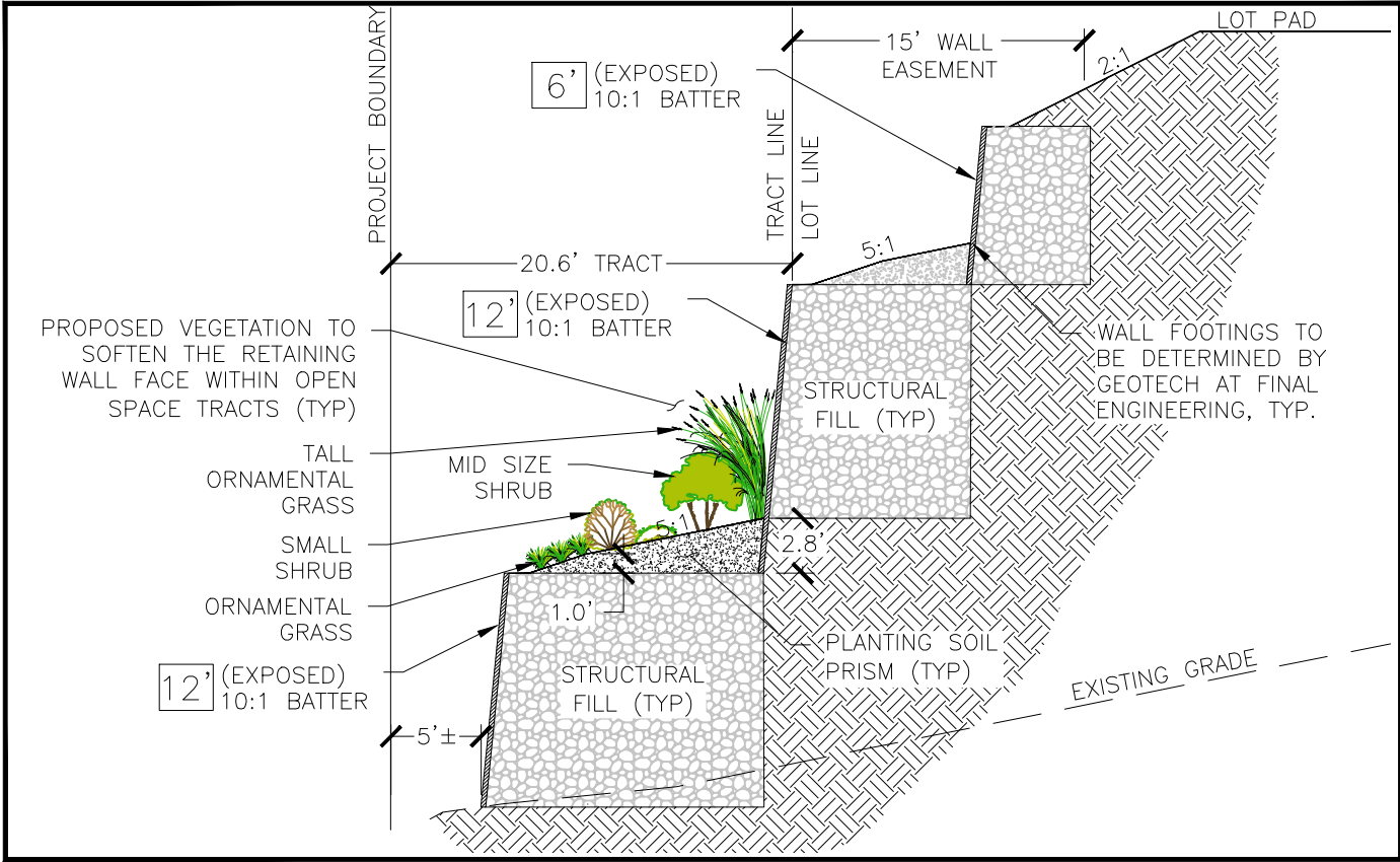
SECTION E-E
