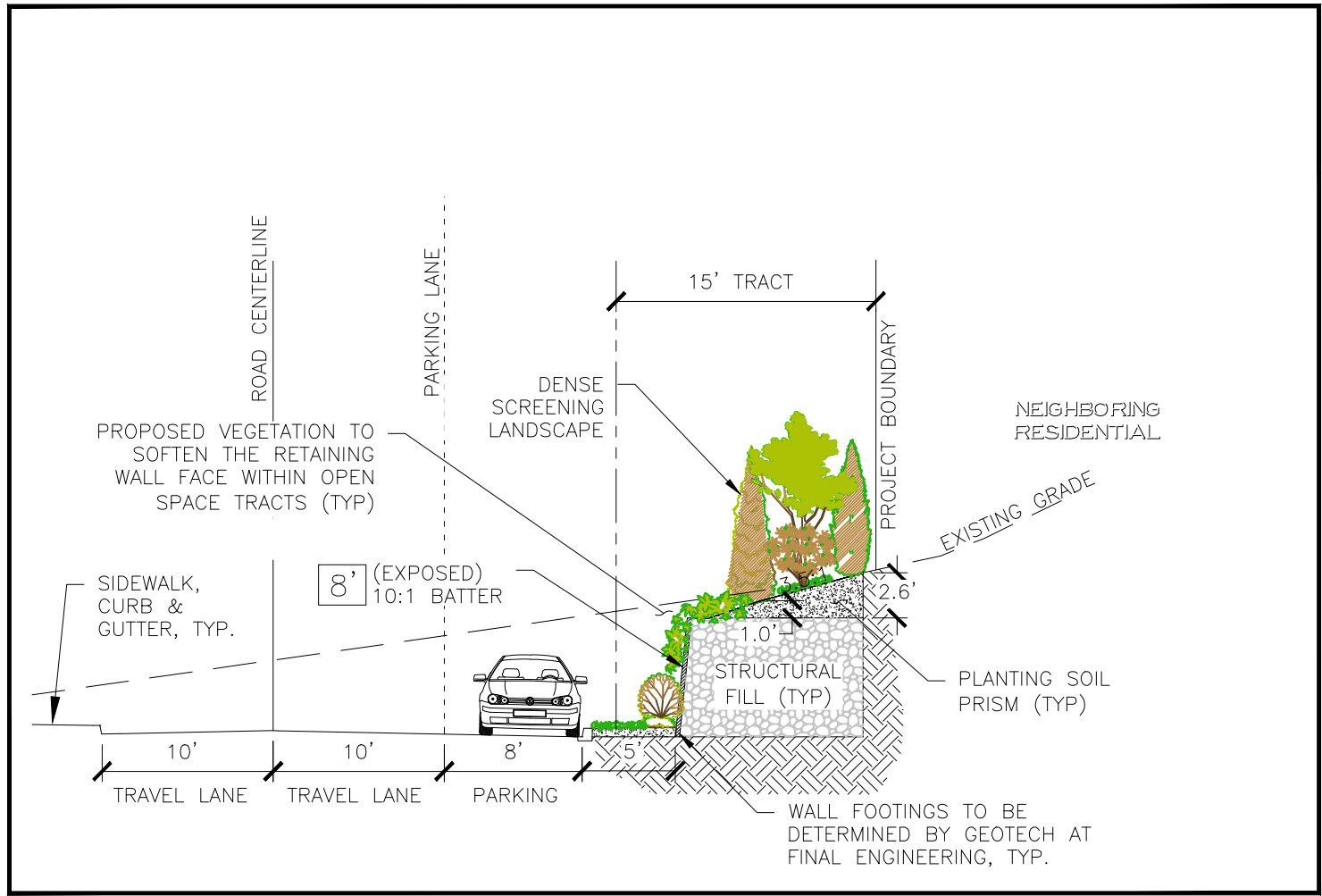
SECTION G-G
