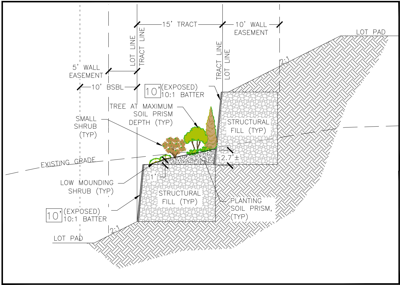
SECTION C-C
